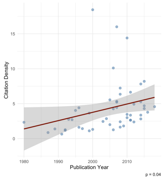
Figure 6. Correlation between Publication Year and Citation Density
